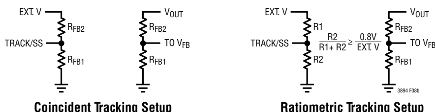
Figure 9(b): Setup for Ratiometric and Coincident Tracking
